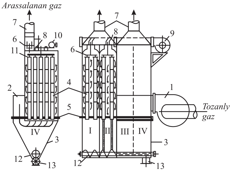
6.5-nji surat. Ýeňli (rukawly) filtr:
